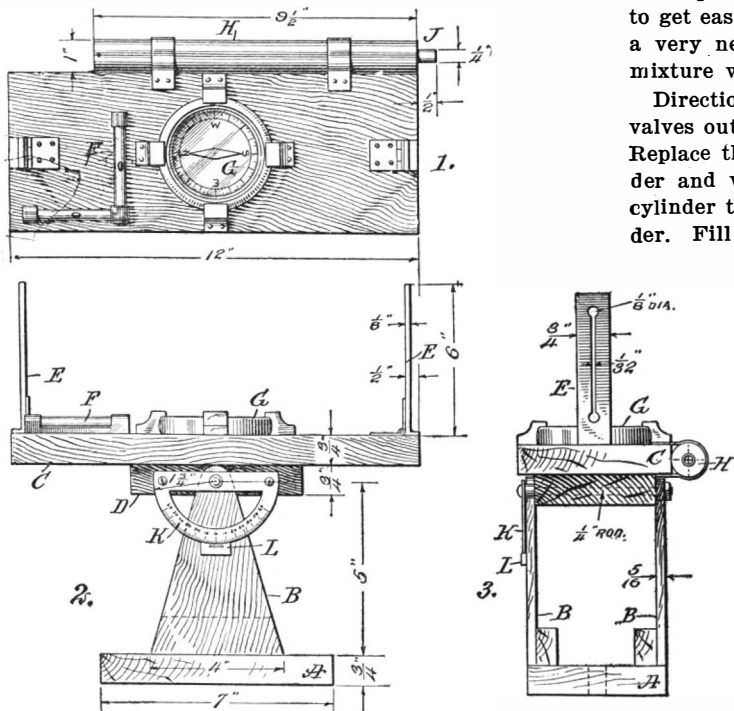
CONSTRUCTIONAL DETAILS OF THE SURVEYING INSTRUMENT.
