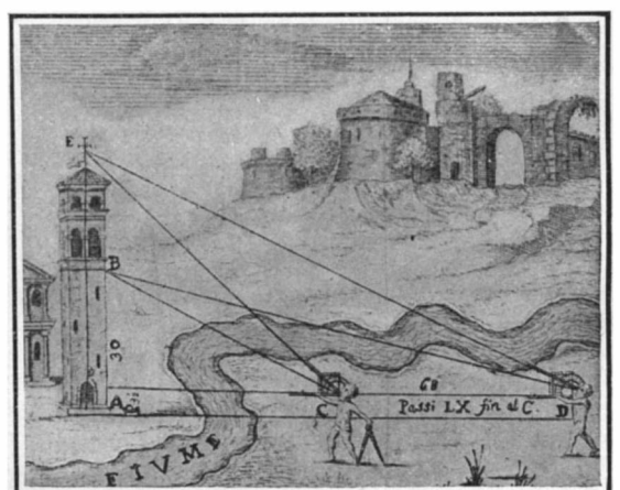
Using the quadrant to measure the altitude of an inaccessible tower.
