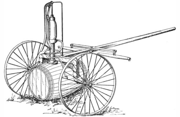
THE HOME-MADE SPRAYER COMPLETE.
