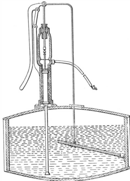
SECTION SHOWING ARRANGEMENT OF AGITATOR.
