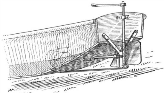
SHAFT BEARING FOR A SMALL BOAT.
