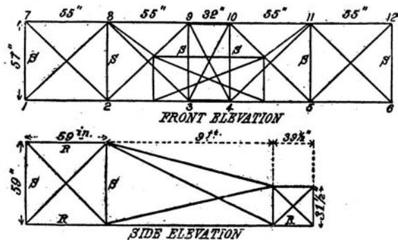
Fig. 1.—Dimensions of the frame.
