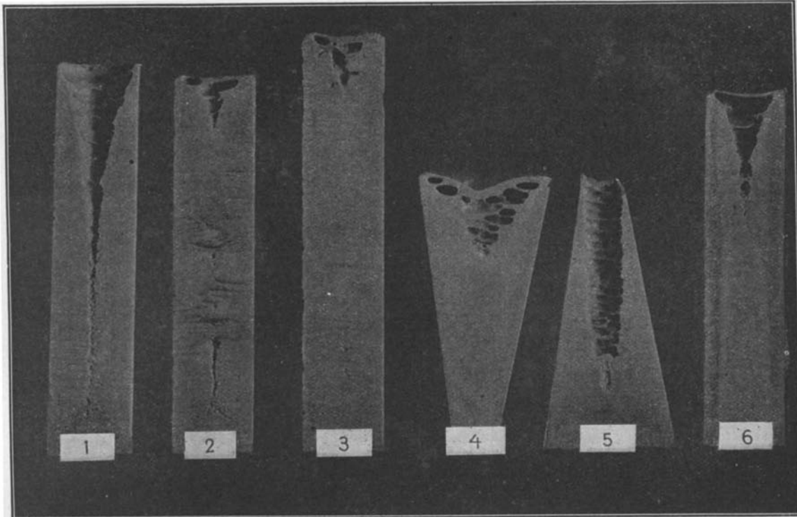
1. Ingot poured rapidly (half a minute); 2, ingot poured fast at first, but slowly afterward; 3, ingot poured very slowly; 4, ingot poured with large end up; 5, ingot poured with small end up; 6, ingot which was kept hot at top and progressively cooled at bottom.
