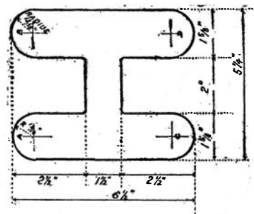
Fig. 8.—Lay-out of clamp for bamboo.
