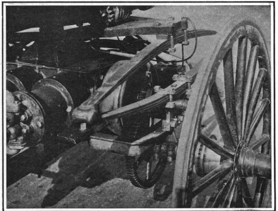
Friction clutch, reducing gears, and hub clutch.
