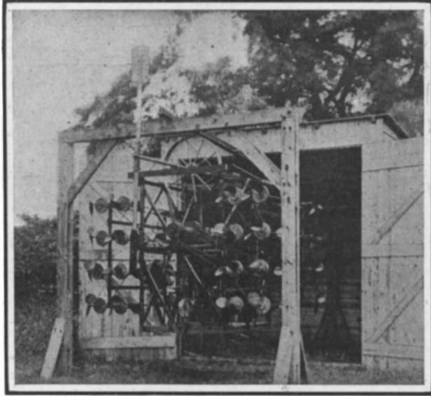
The small propellers which collectively take the place of the single 9-foot large propeller are mounted on 1/4-inch shafts, three on a shaft, with eight shafts on each side of the framework of the car. All eight shafts are driven by round leather belting and pulleys from the central countershaft. The aggregate area of the small propellers is 19 square feet. That of the single big propeller is 2 square feet.
