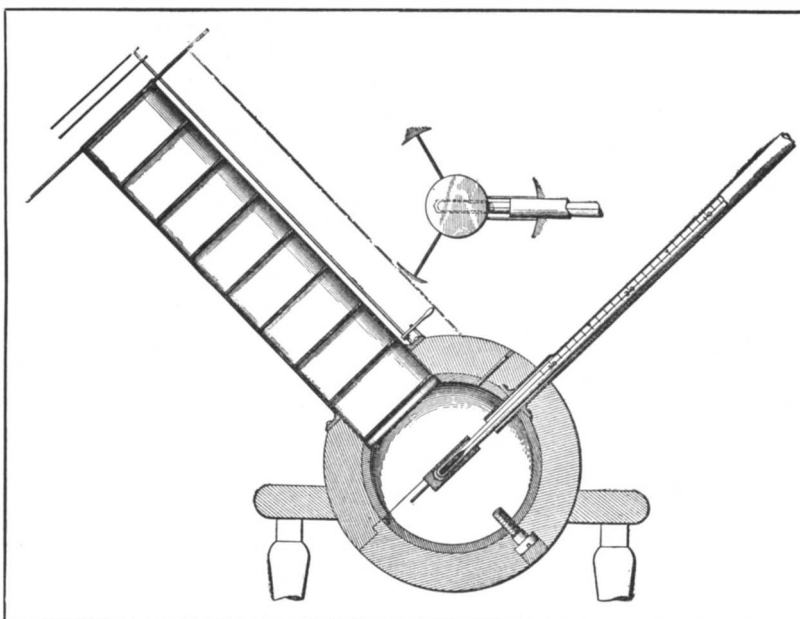
Details of the Pyrhelimeter.
