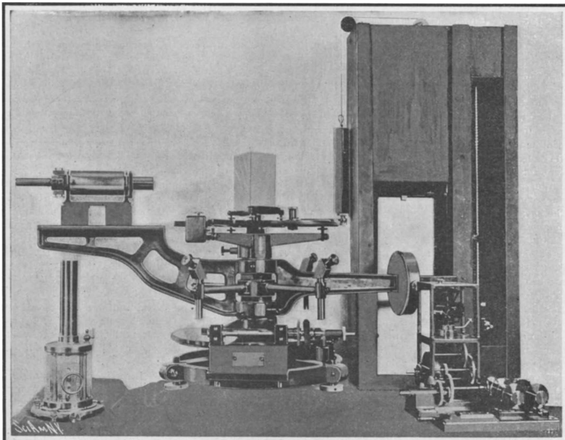
The Spectrolometer, an Instrument that Measures the Energy in Various Parts of the Solar Spectrum.
