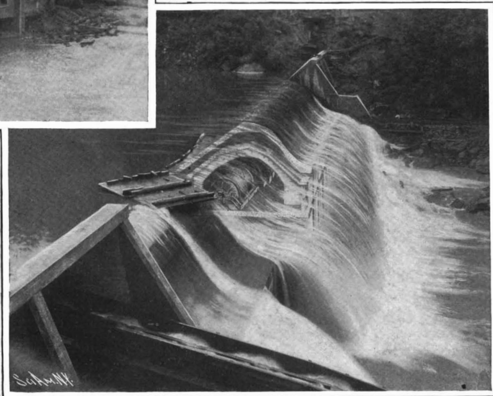
View Looking Along Axis of Dam, with Portion of Apron Broken Away to Show Position of Waterwheels Within the Dam.
