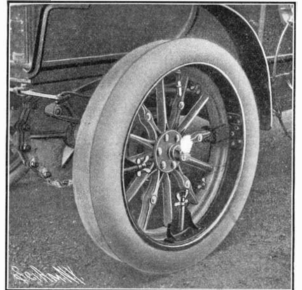
NOVEL SPARE WHEEL AND TIRE DEVICE FOR AUTOMOBILES.
