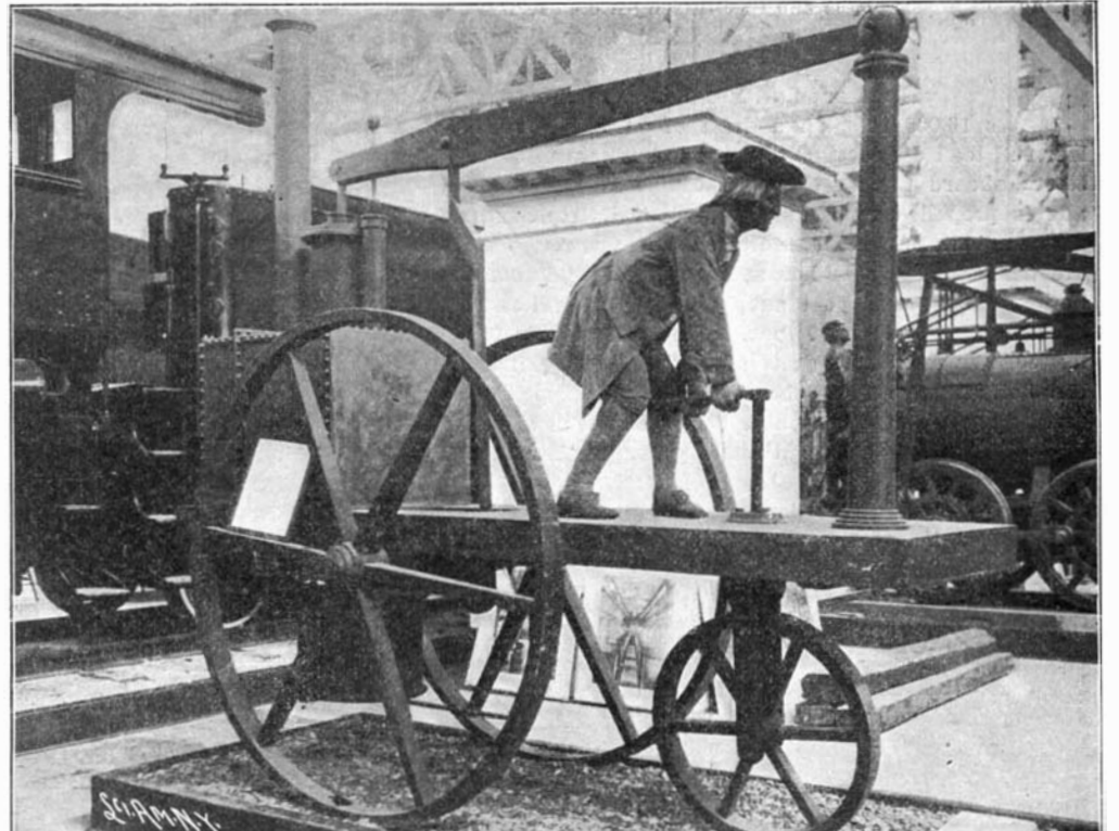
Fig. 6.—Murdock's Road Locomotive, 1784.
