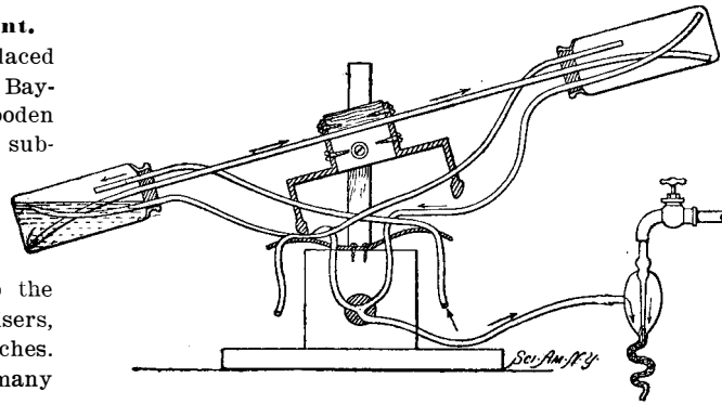
AN IMPROVED MICHAUD APPARATUS.
