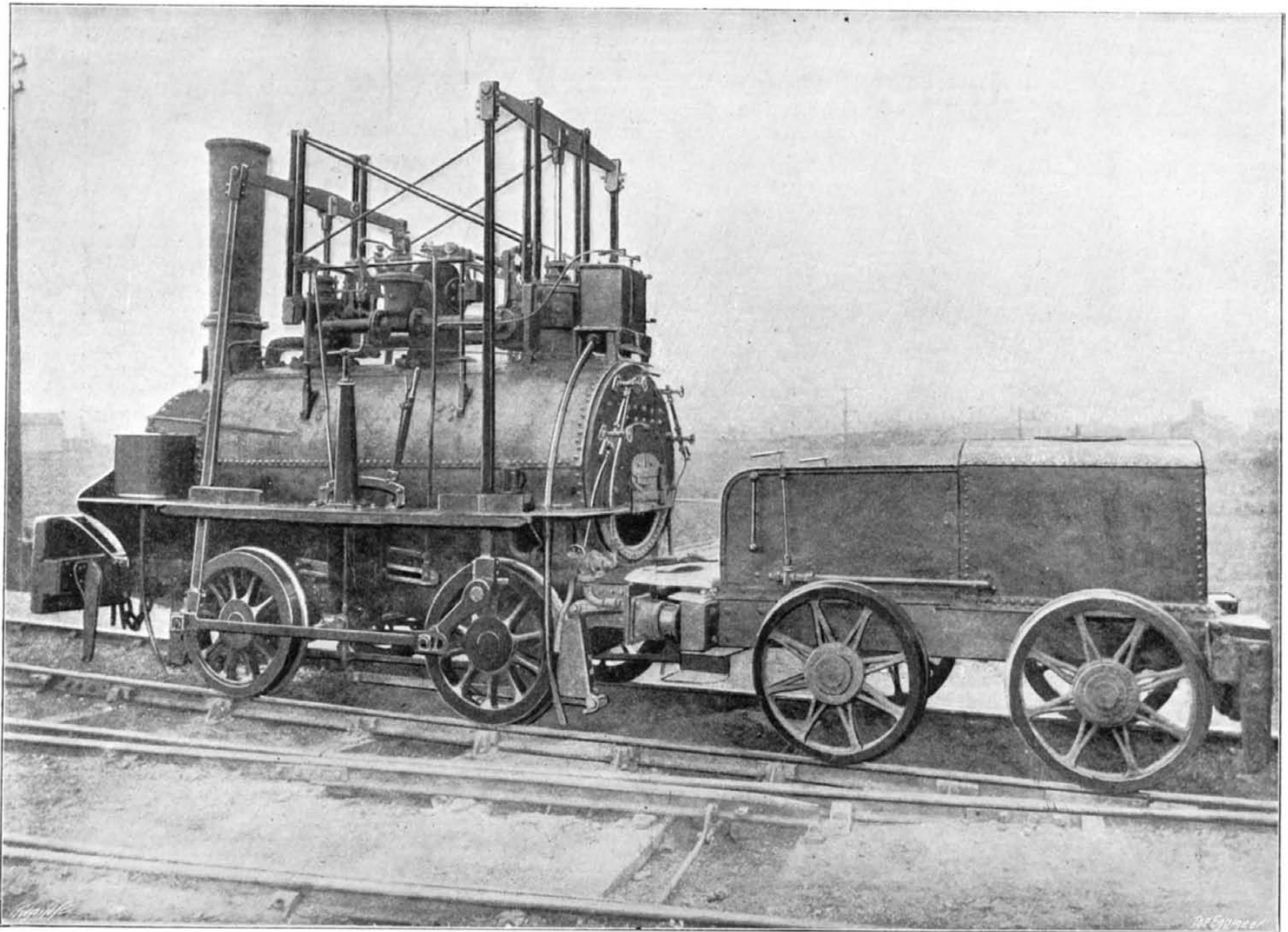
Built by George Stephenson in 1822 and only lately removed from service. Cylinders, 10 \frac{3}{4} inches diameter by 24 inches stroke. Weight, 15 tons.
