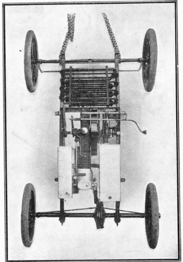
Plan View of the Oldsmobile.
