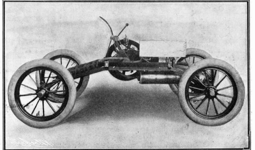
Carriage Body Removed, Showing Running Gear and Motor.
