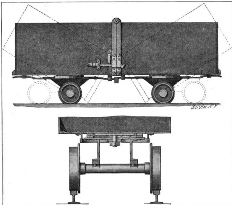
IMPROVED DUMPING CAR.
