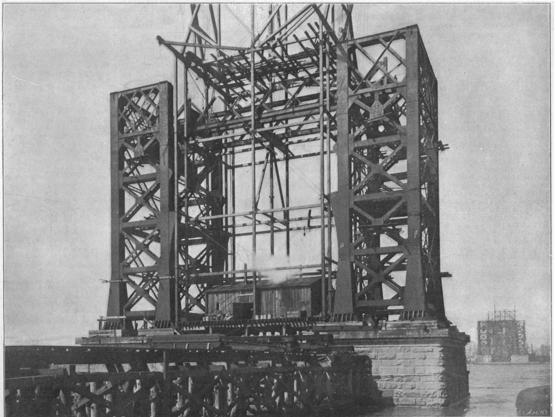
Size of Base, Center to Center of Columns, 24 feet by 40 feet. Section of Columns at Base, 8 feet by 8 feet.— Height of Towers, Top of Masonry to Center of Cables, 310 feet. Clear Span of Bridge, 1,600 feet.
