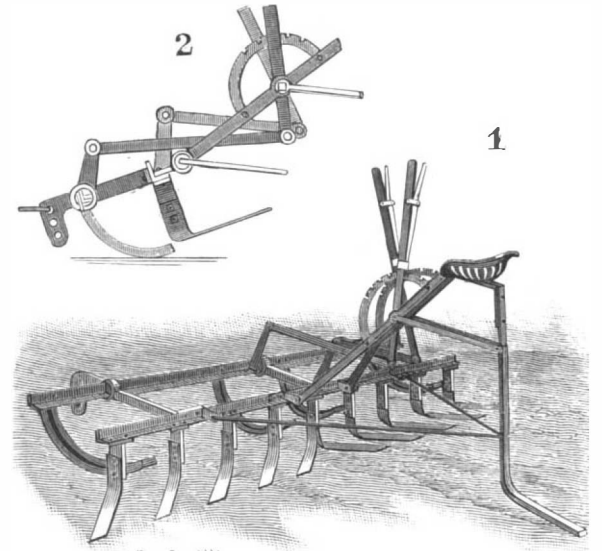
GUNNINGS'S WEEDING-MACHINE.
