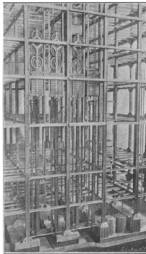
DETAILS OF FOUNDATIONS, SIDEWALK, AND ELEVATORS.
