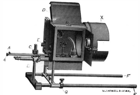
Fig. 5.—OXYHYDROGEN BURNER.
