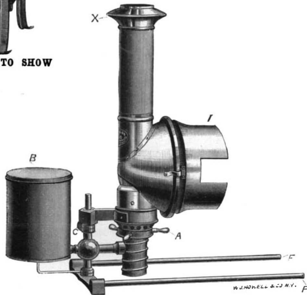
Fig. 4.—OIL BURNER.
