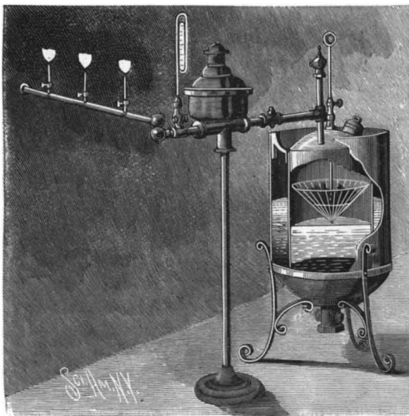
SECTION OF GAS EVOLUTION APPARATUS.
