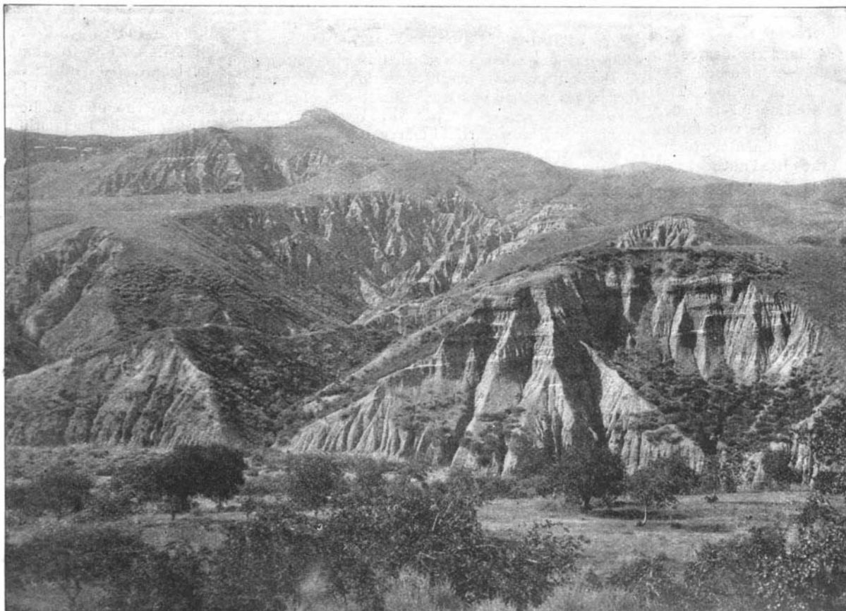
RECENT GEOLOGICAL ACTION, SANTA CLARA-SAN BENITO VALLEY, CAL.
