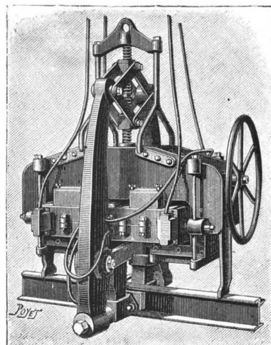
Fig. 3.—WELDING TRANSFORMER.
