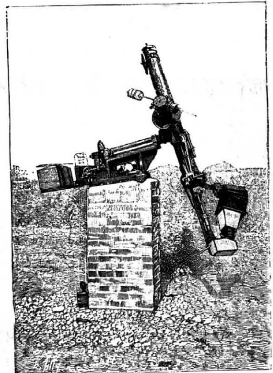
APPARATUS FOR MEASURING THE ROTATION OF THE CORONA.
