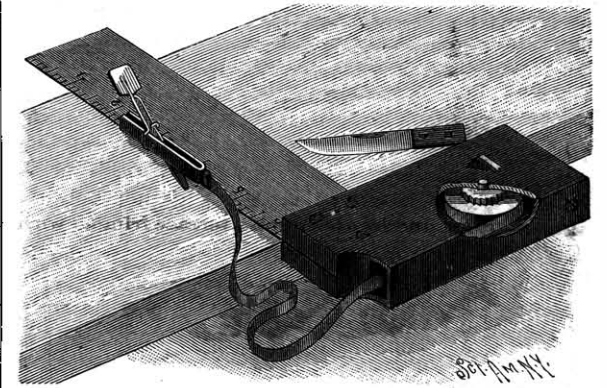
DUNNINGTON'S CARPENTER'S SQUARE.
