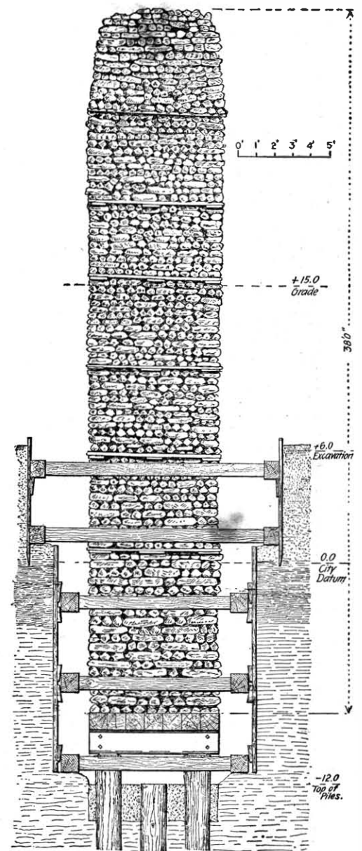
METHOD OF TESTING FOUNDATION PILES OF PUBLIC LIBRARY BUILDING, CHICAGO.
