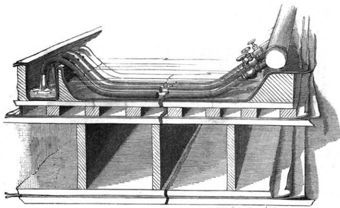
FLOOR AND BRINE PIPING ARRANGEMENT.
