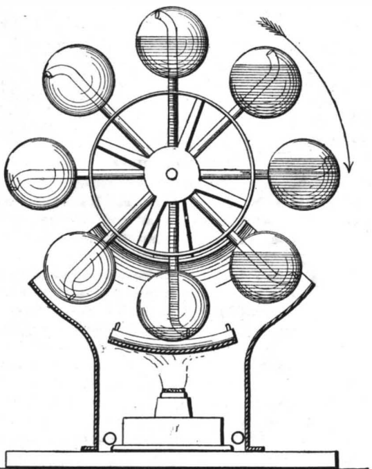
ISKE'S HEAT MOTOR—AMERICAN PATENT.
