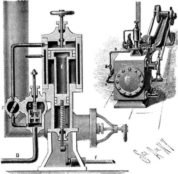
MCIHENNY'S STEAM ENGINE GOVERNOR.
