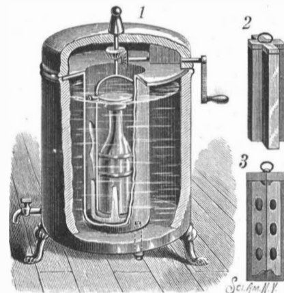
DERMIGNY'S FAMILY ICE MACHINE.
