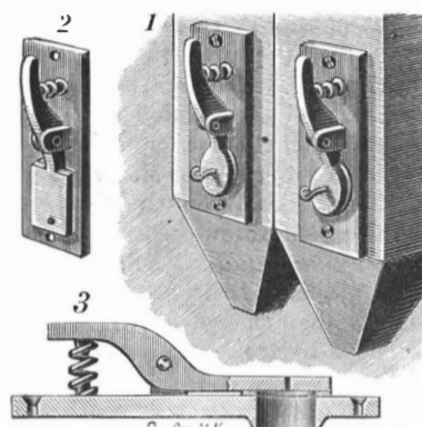
GIRARDIN'S ORGAN PALETTE.
