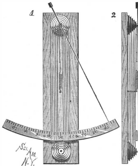
Fig. 1.—METALLIC THERMOMETER.
