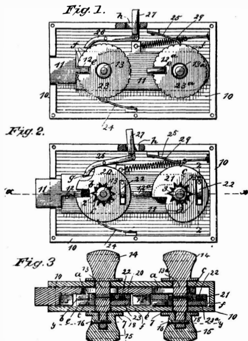
DOUGLASS' COMBINATION LOCK.
