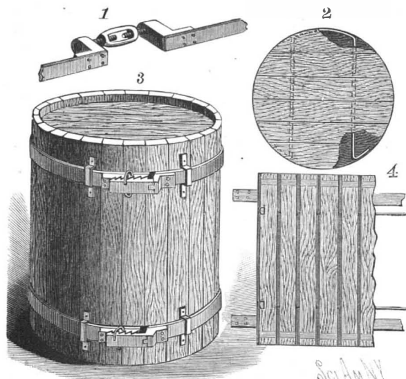
MITCHELL'S COLLAPSIBLE SHIPPING CASK.
