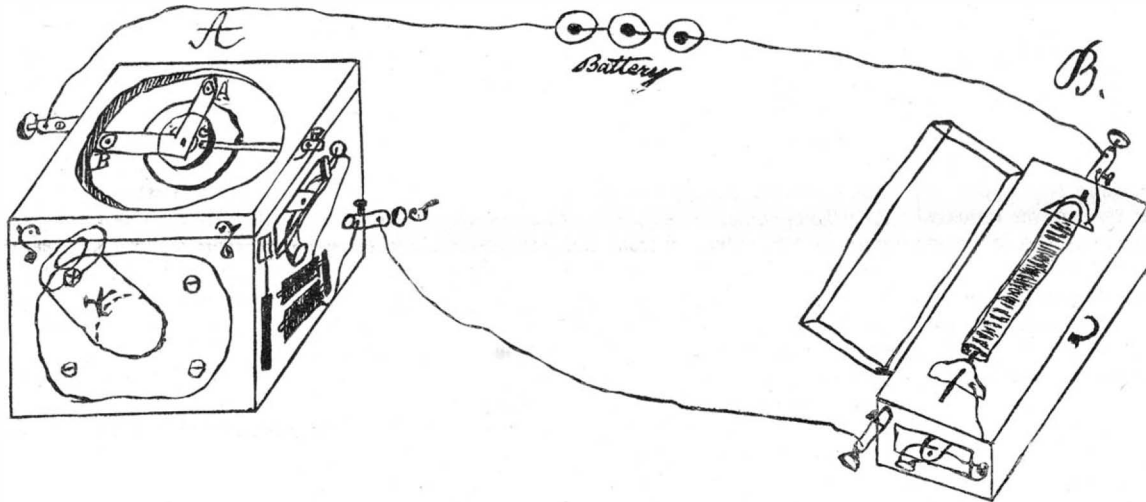
SKETCH OF THE FIRST TELEPHONE, AS MADE BY THE INVENTOR.
