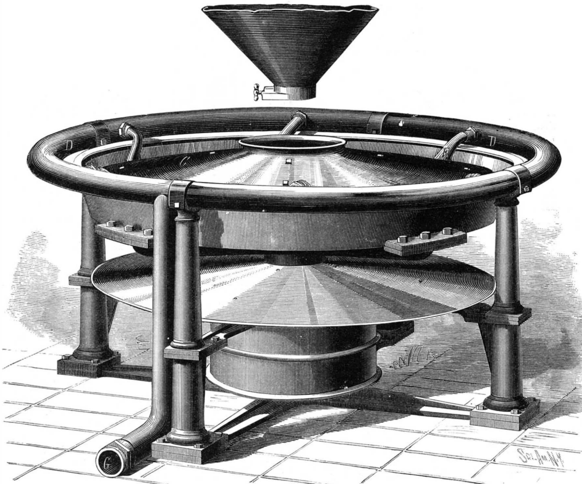
HENWOOD'S ORE SEPARATOR.
