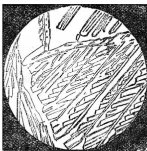
Fig. 2.—Potassium Nitrate.
