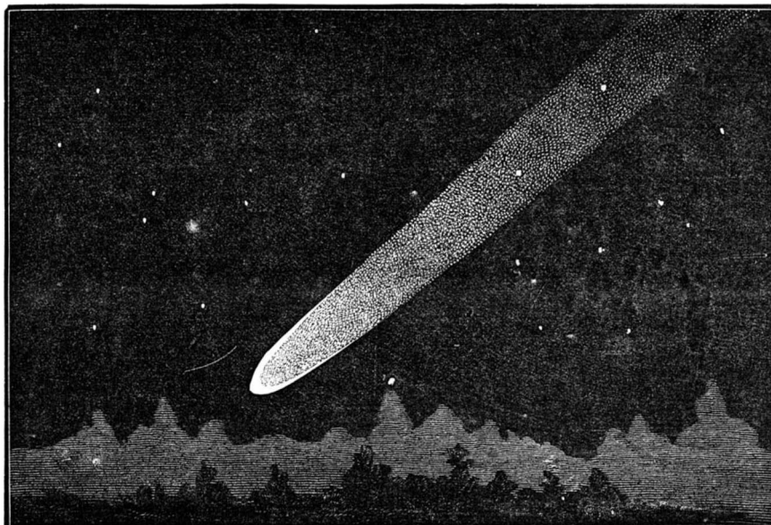
COMET ACCORDING TO BROOKS' SKETCH.
