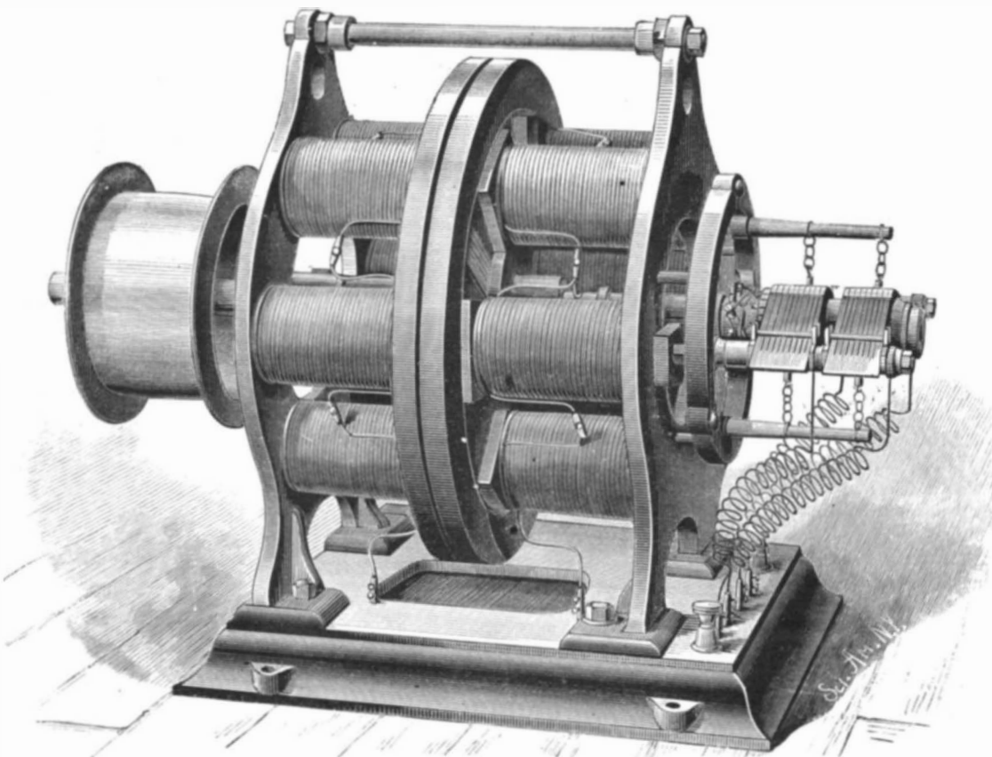
Fig. 2.—COMPOUND MULTIPOLAR CONTINUOUS-CURRENT MACHINE.
