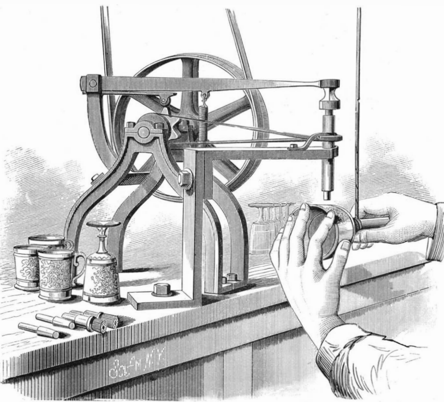
MACHINE FOR ORNAMENTING METAL SURFACES.
