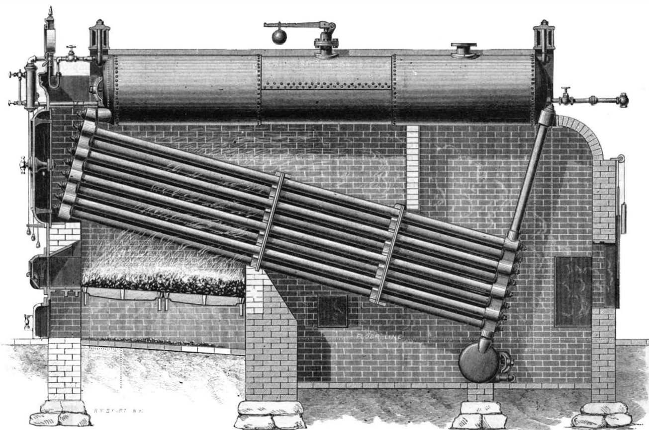
FIG. 1.—SIDE ELEVATION OF THE BABCOCK & WILCOX WATER TUBE BOILER.
