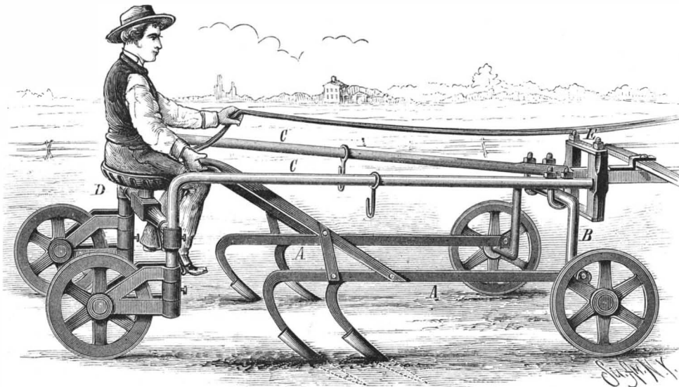
COLE'S RIDING ATTACHMENT FOR CULTIVATORS.
