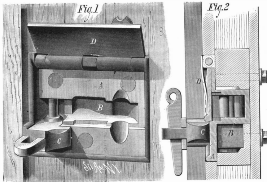
BUSER & SHAW'S CAR DOOR FASTENER.
