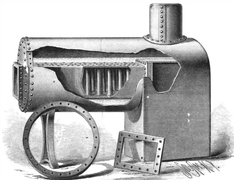
OGLE AND BURNETT'S IMPROVED BOILER.
