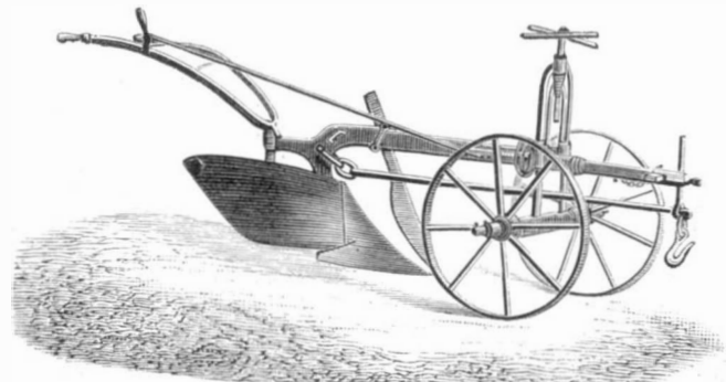
Fig. 8.—DURAND'S BRABANT SIMPLE.
