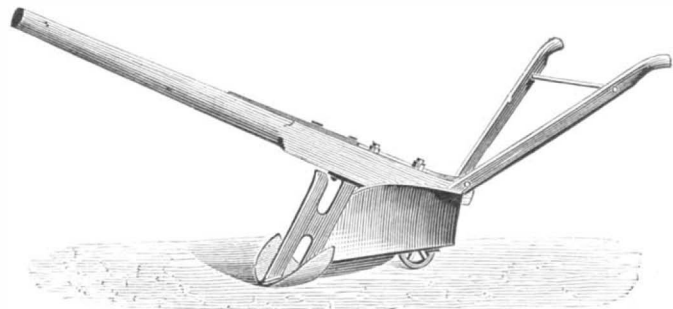
Fig. 24.—BILLOT'S TRENCHING PLOW.
