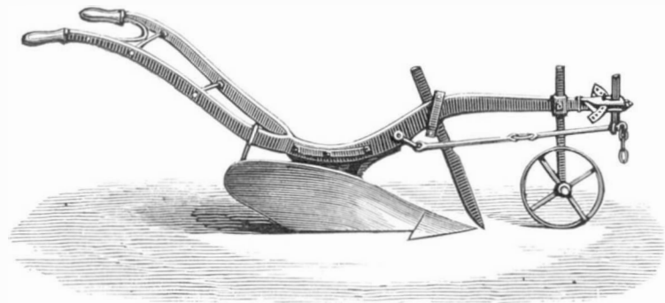
Fig. 2.—FRENCH ONE-WHEEL PLOW.
