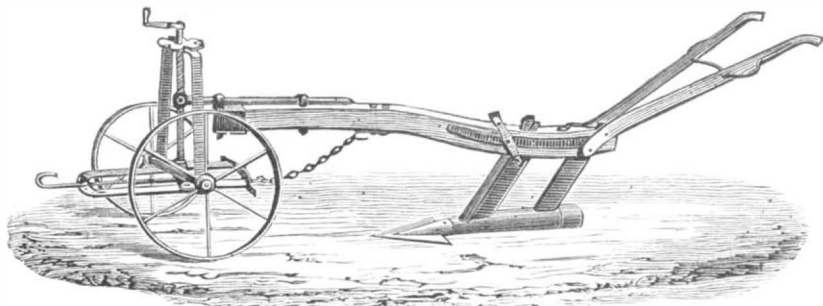
Fig. 25.—MOLE PLOW.
