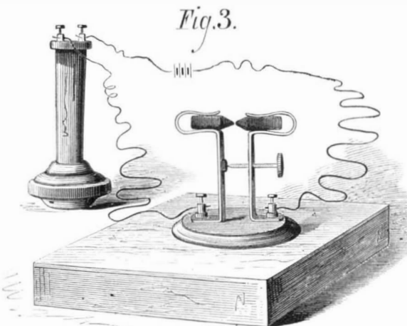
Fig. 3.—MICRO-TELEPHONE ON A PLAIN SOUNDING BOARD.
