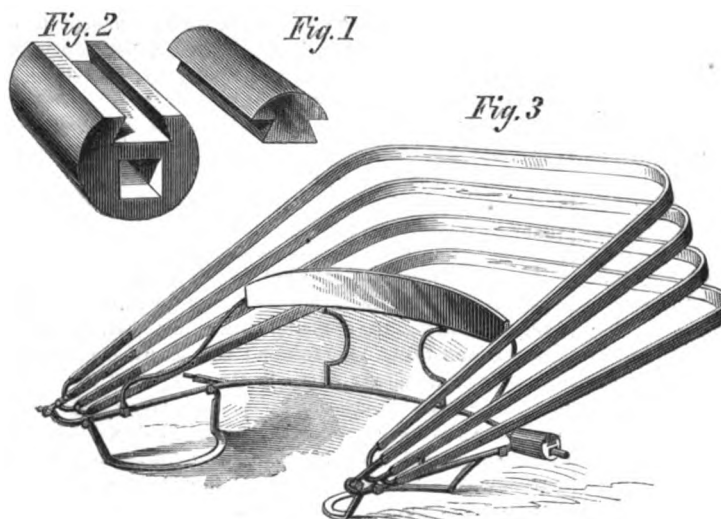
STICKEL'S IMPROVED PROP BLOCK.
