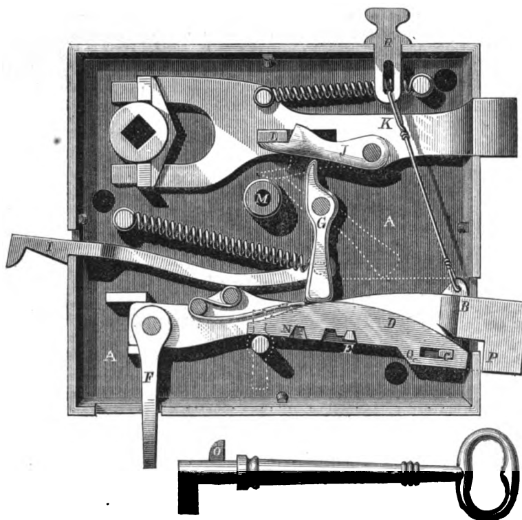
MILLER'S COMBINED BOLT AND LOCK.
