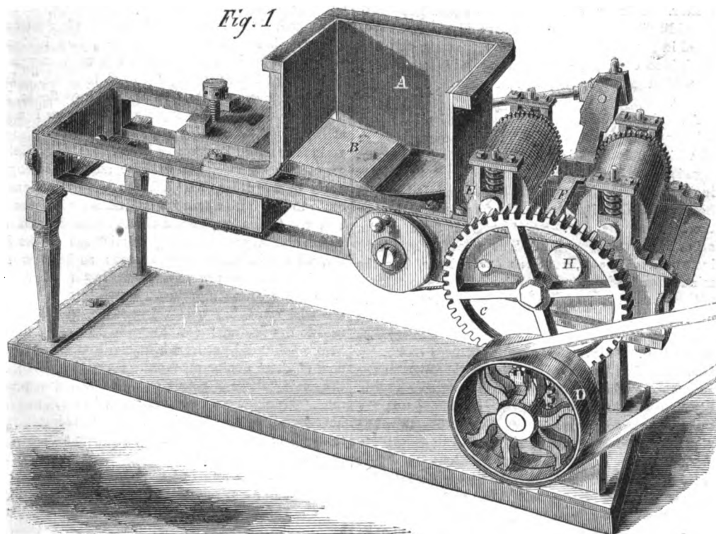
CONNETT'S SHINGLE MACHINE.
