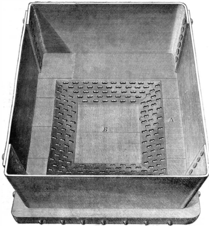
LISTER'S GRATE FOR LOCOMOTIVE FIRE-BOXES
