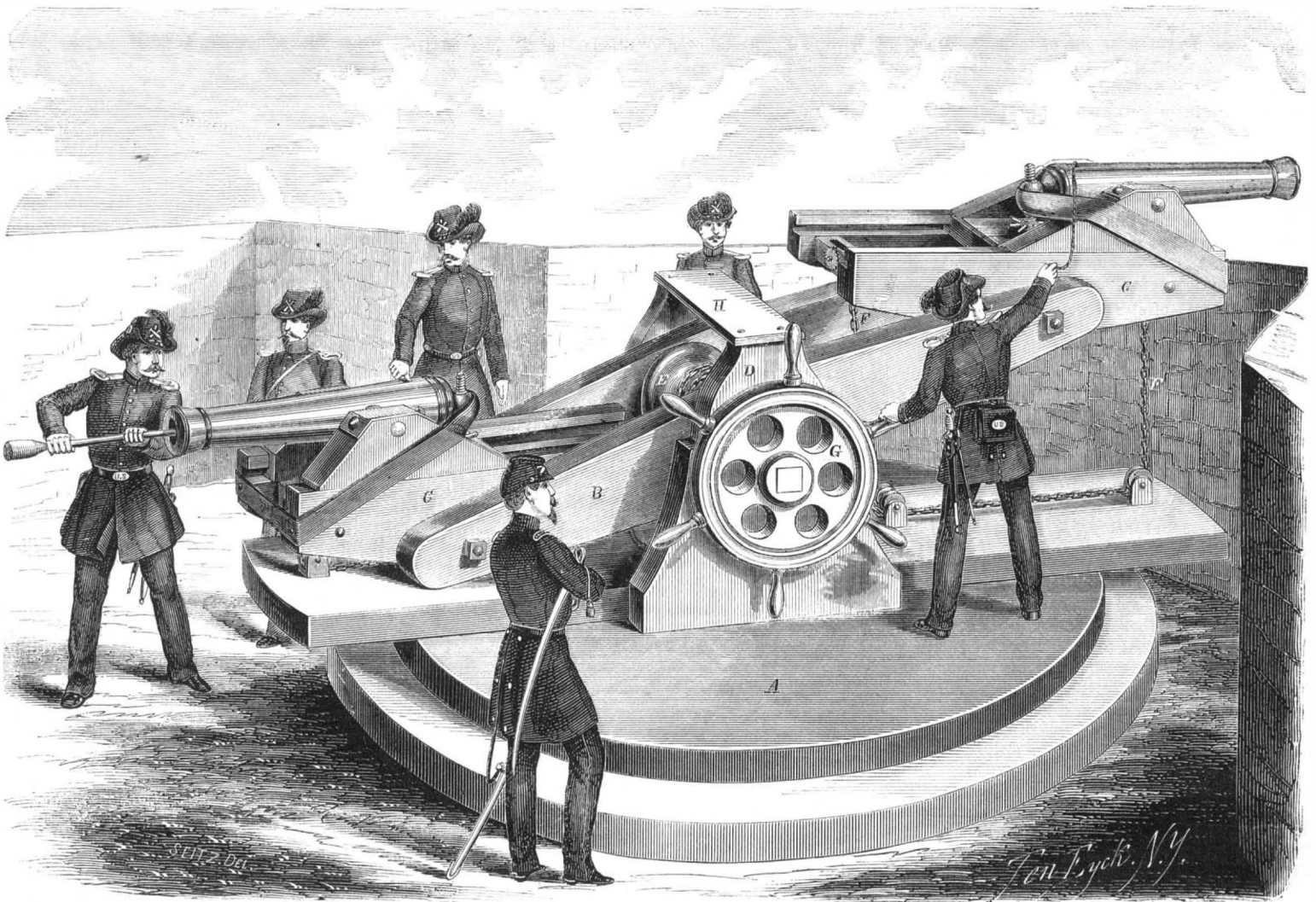
HOPKINS'S IMPROVED MODE OF MOUNTING CANNON.
