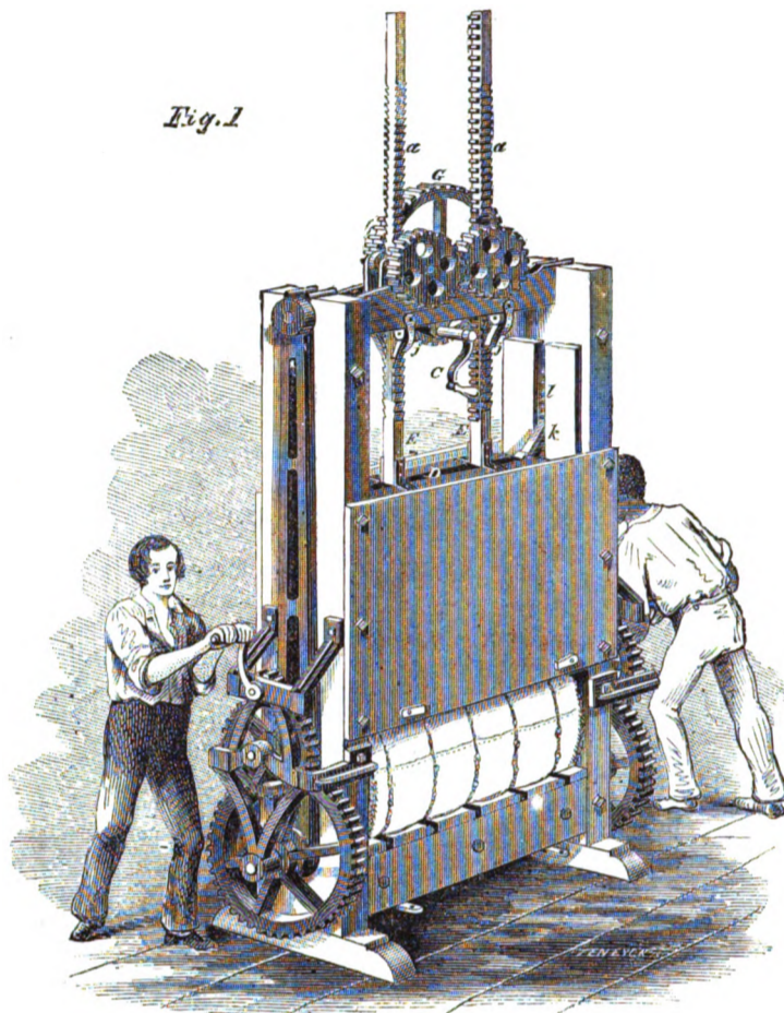
RANDEL'S IMPROVED COMBINATION PRESS.
