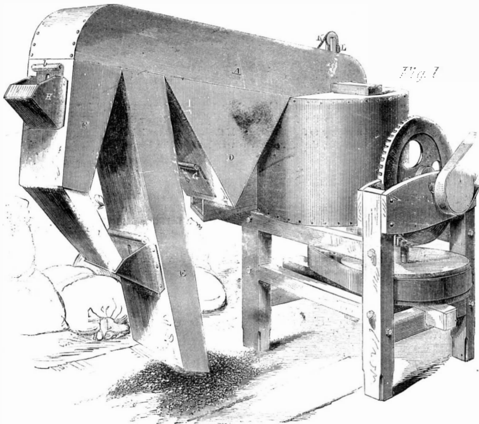
COX'S IMPROVED GRAIN SEPARATOR.
