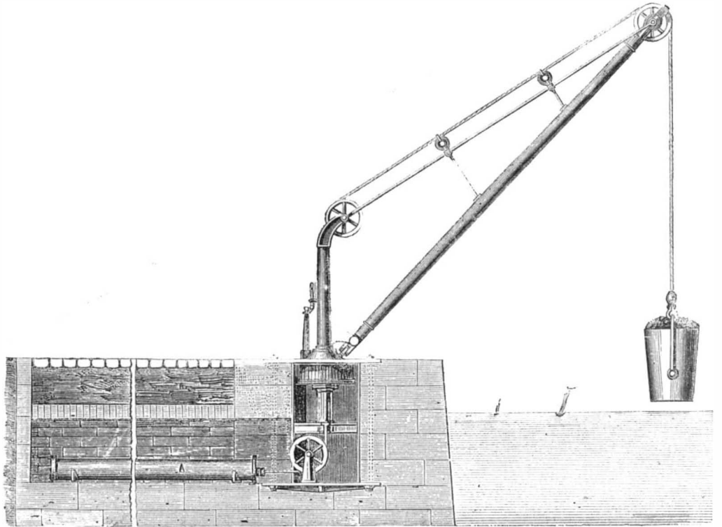
NEW STEAM CRANE.
