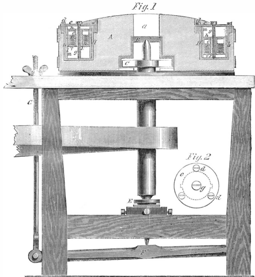
FAIRCLOUGH'S MILLSTONE BALANCE.
